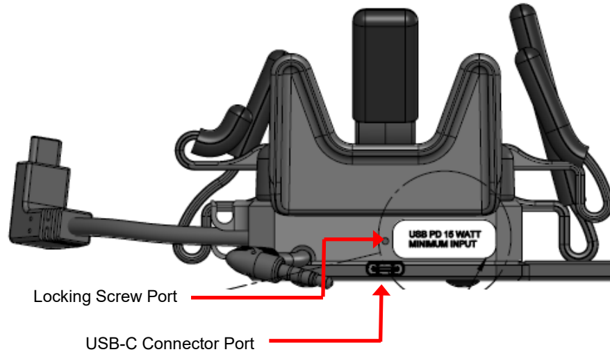
Figure 142: Cradle Assembly – Bottom View
